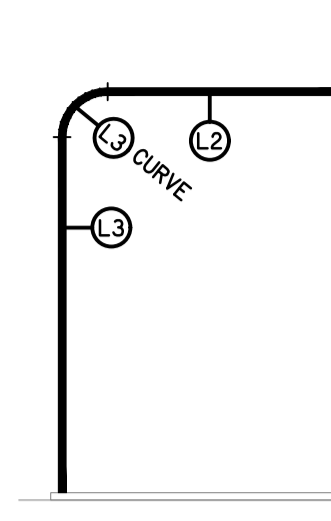
DETAIL E L3 / L2 LIGHTING SECTION SCALE 1:50
