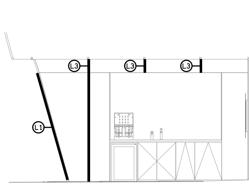
DETAIL C L3 LIGHTING ELEVATION SCALE 1:50
